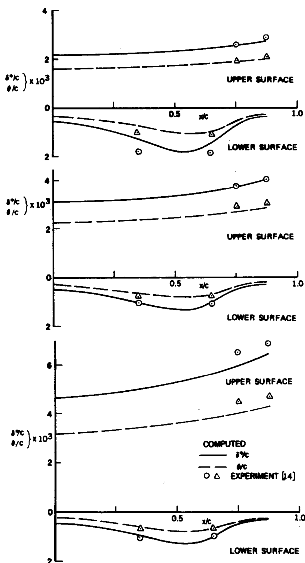
Fig. 5 Comparison of calculated and measured boundary-layer parameters of case 2.
