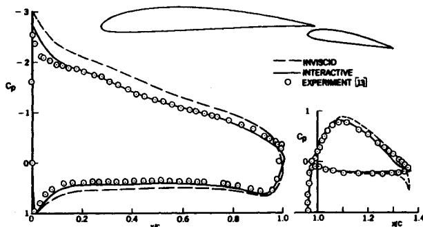
Fig. 1 Comparison of calculated and measured pressure distribution for the data of Olsen and Orloff. 13
