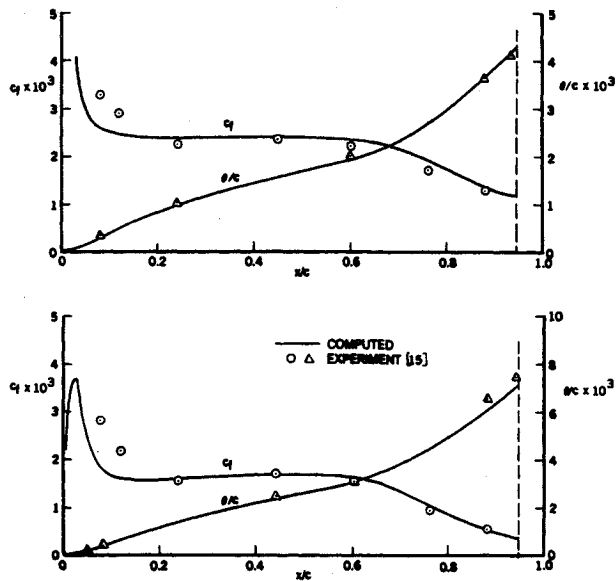
Fig. 8 Comparison of calculated and measured skin-friction coefficient and momentum thickness ( \theta/c ) on the NLR 7301 wing upper surface: a) \alpha = 6 deg, b) \alpha = 13.1 deg.
