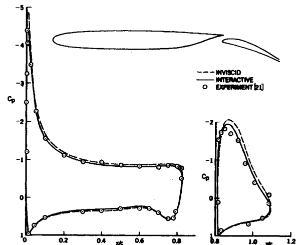
Fig. 2 Comparison of calculated and measured pressure distribution on case 2 for \alpha = 0 deg.
