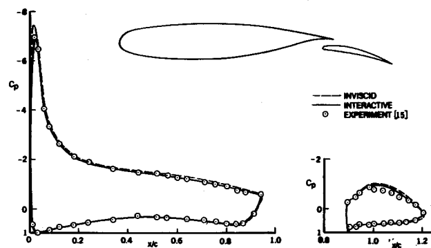
Fig. 6 Comparison of calculated and measured pressure distribution on the NLR 7301 wing and flap for \alpha = 6 deg.
