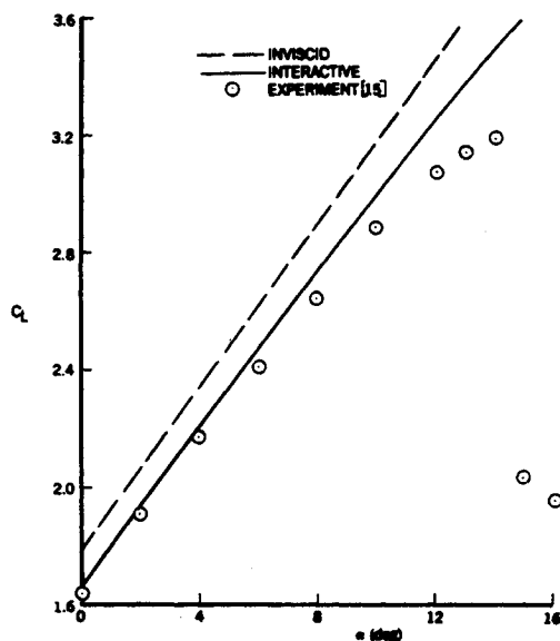
Fig. 9 Comparison of calculated and measured lift coefficient of NLR 7301 wing with flap.
