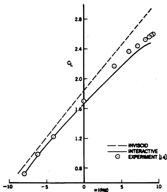
Fig. 4 Comparison of calculated and measured lift coefficient, C_L of case 2.
