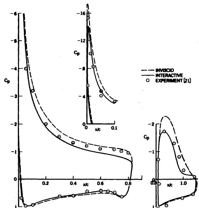
Fig. 3 Comparison of calculated and measured pressure coefficients of case 2 for \alpha = 8.93 deg.
