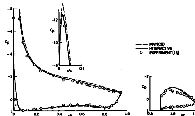
Fig. 7 Comparison of calculated and measured pressure distribution on the NLR 7301 wing and flap for \alpha = 13.1 deg.
